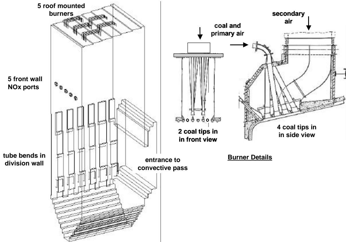
Figure 6. Schematic of the half furnace model and detail of a multi-tip burner from the furnace. In the burner front view, two coal tips fire through six gaps between roof tubes (adapted from Babcock and Wilcox Company, 1963).
