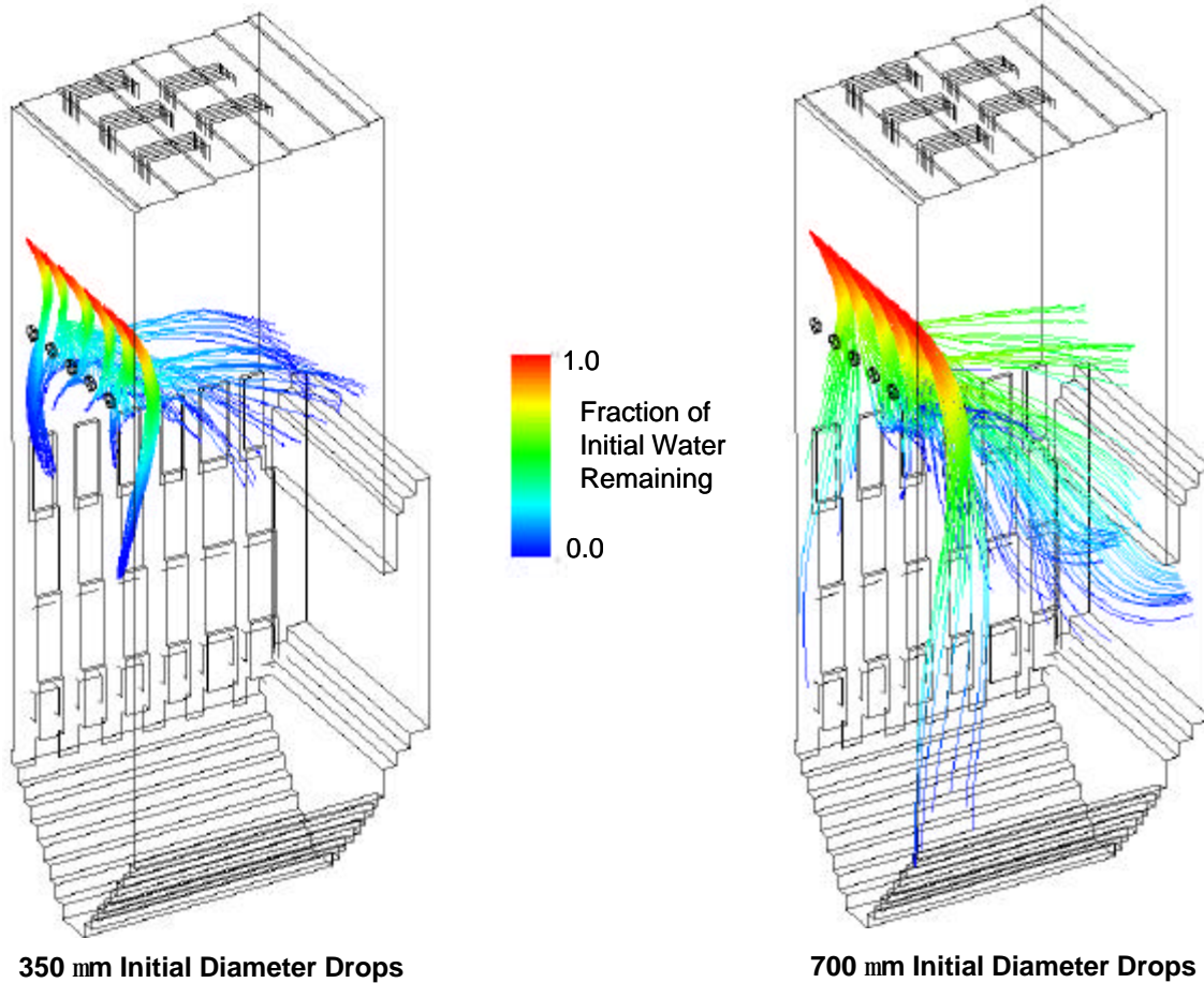
Figure 10. Predicted water droplet trajectories for 350 mm and 700 mm initial diameter drops.
