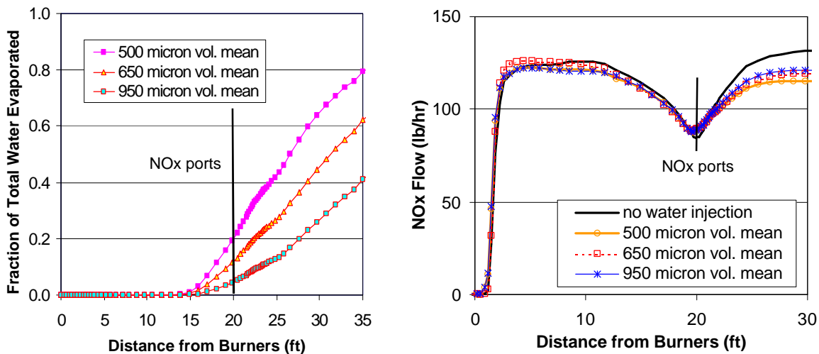
Figure 11. Plots of the cumulative fraction of injected water evaporated (left) and downward NO x flow (right) vs. distance below the burners.
