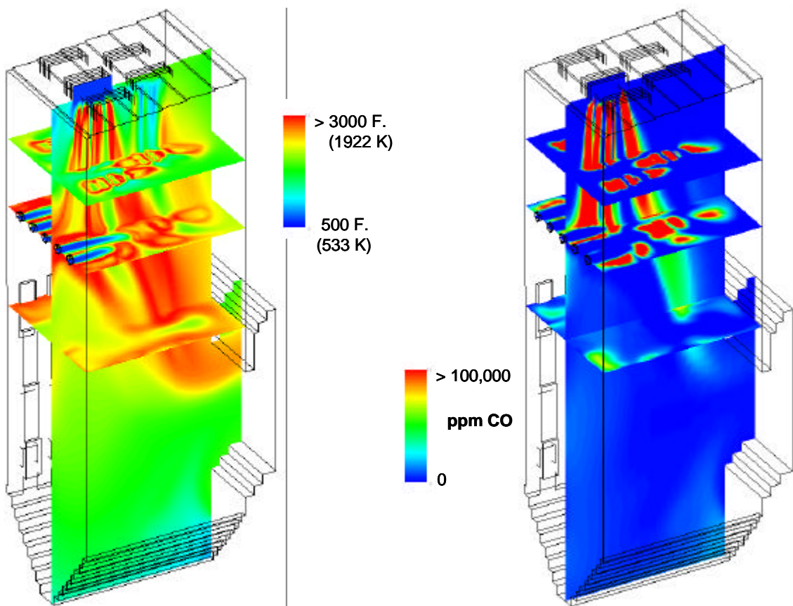
Figure 7. Predicted flue gas temperature and CO concentration for the baseline furnace model.
