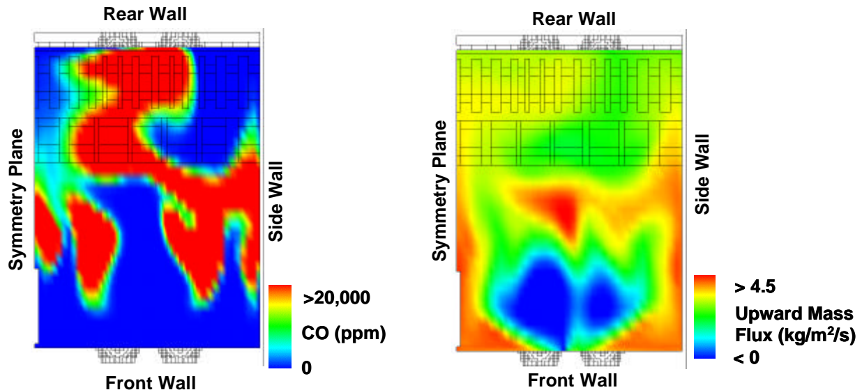
Figure 3. Plots of CO concentrations (left) and upward flue gas mass flux (right) at proposed OFA elevation.
