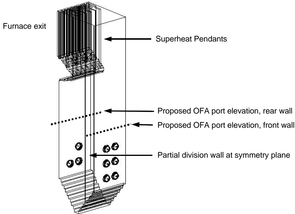
Figure 2. Schematic of half furnace model for opposed wall fired boiler showing OFA port elevations.
