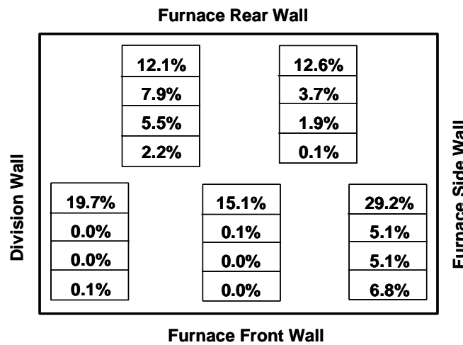
Figure 8. Predicted carbon in fly ash for coal originating from each of the four pairs of coal tips in each of the five burners in the half furnace model.
