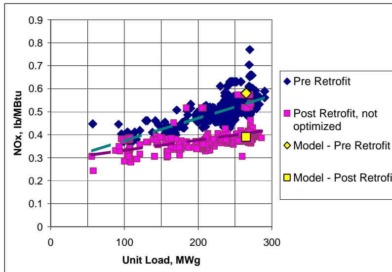
Figure 5. Comparison of predicted and reported NOx emission rates before and after OFA retrofit.
